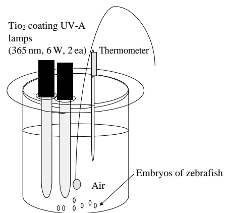
Fig. 2. Photo catalytic reactor used for coated TiO 2 toxicology tests.
